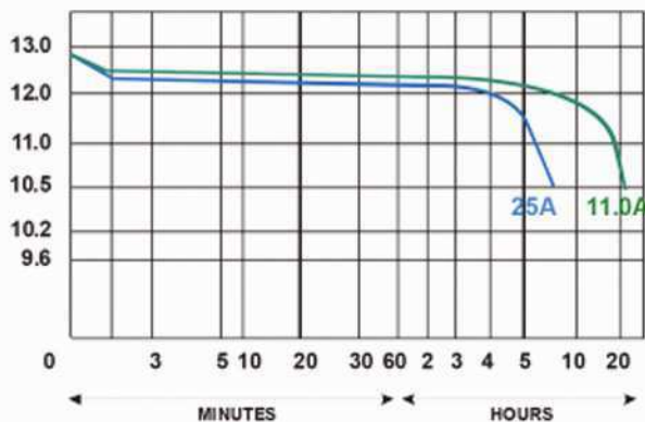
25A and 20 hour discharge characteristics
